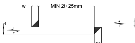
TYPICAL LAP WELD
