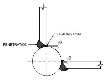
CHINE BAR CONNECTION-1
