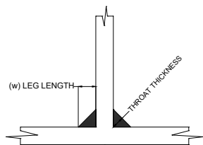
TYPICAL FILLET
